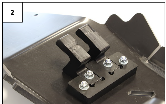
2 4 Tfhc 6x30mm + 4 M6 Washers + 4 Em6f
