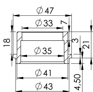
S.s. Bushing Cod.204870R
