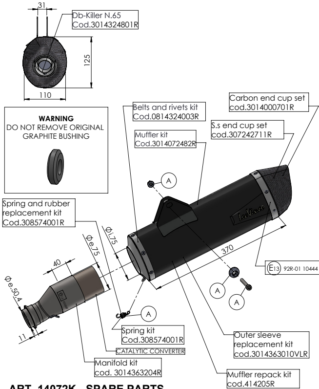
ART. 14072K - SPARE PARTS
