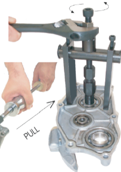
Bridge type turning operation
