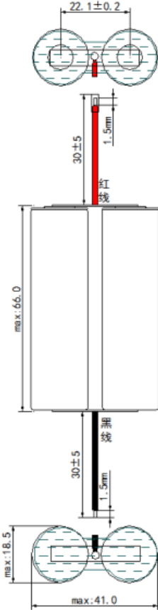
Battery: Max. 18.5mm (T) x Max. 41.0mm (W) x Max. 66.0mm (L)
